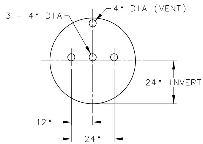
BAFFLE DETAIL
